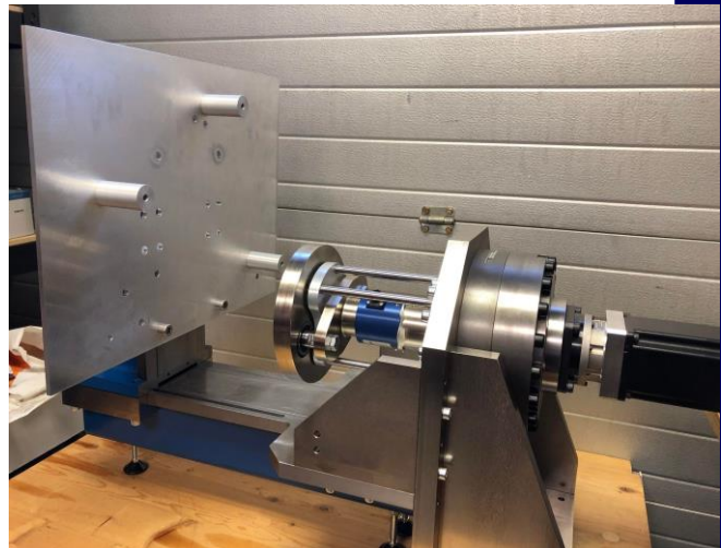
UTCM with Tool Tester Extension and Vertical Mounted Torque Tester fittings.
